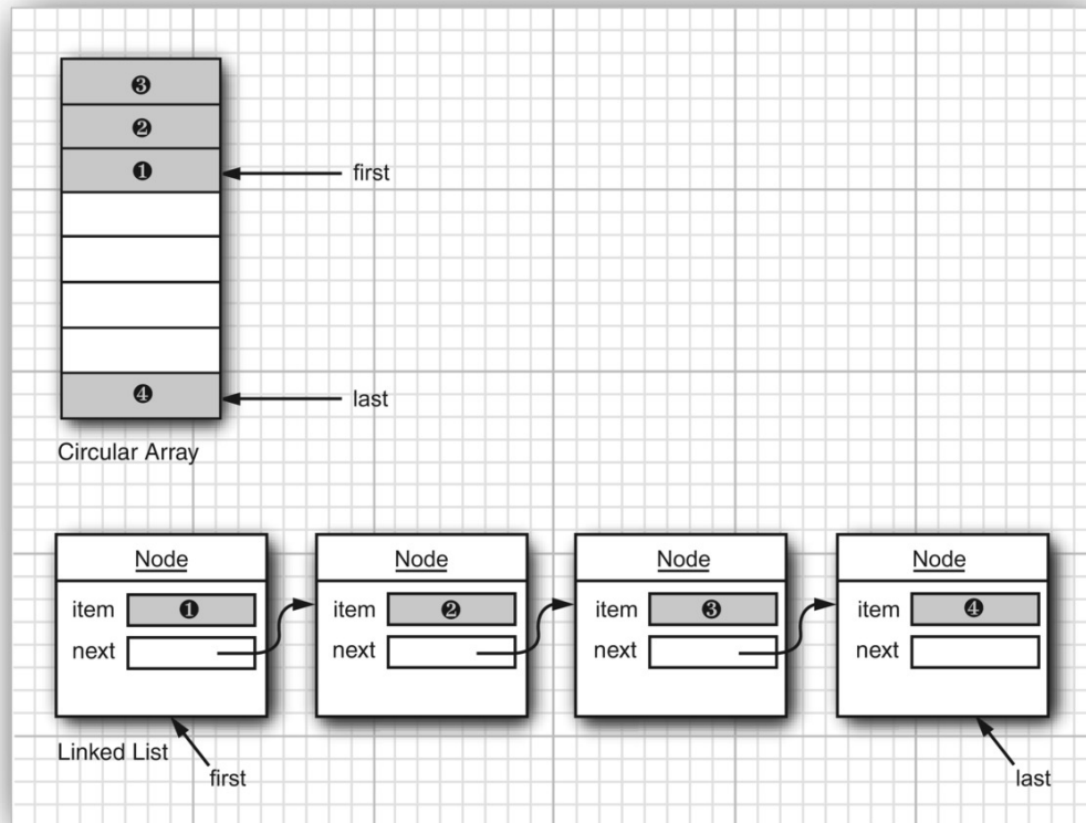
Figure 9.2: Queue implementations
