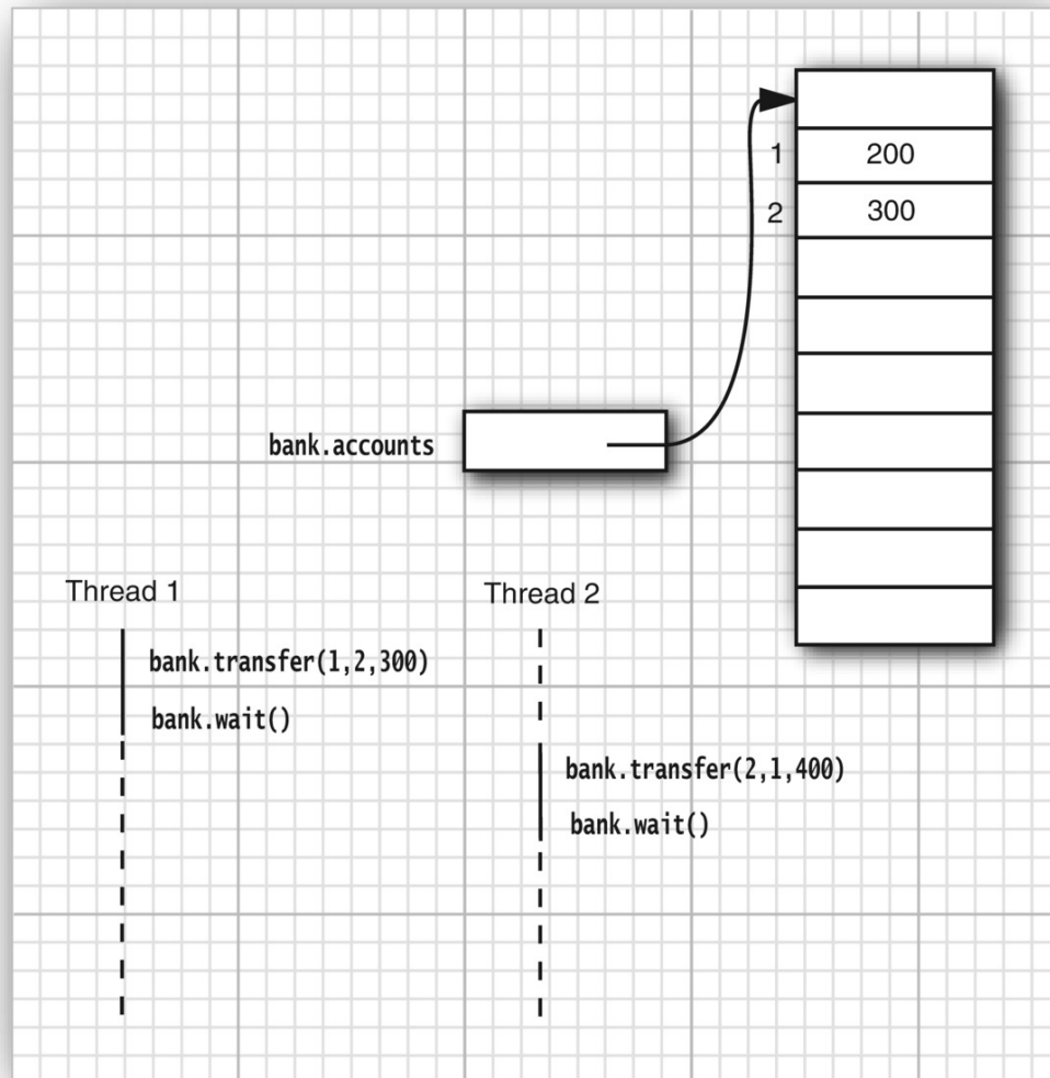
Figure 10.4: A deadlock situation
