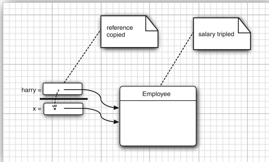
Figure 4.7: Modifying an object referenced by a parameter has a lasting effect.
