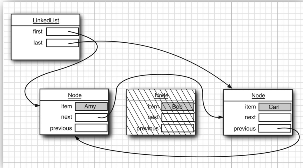
Figure 9.8: Removing an element from a linked list
