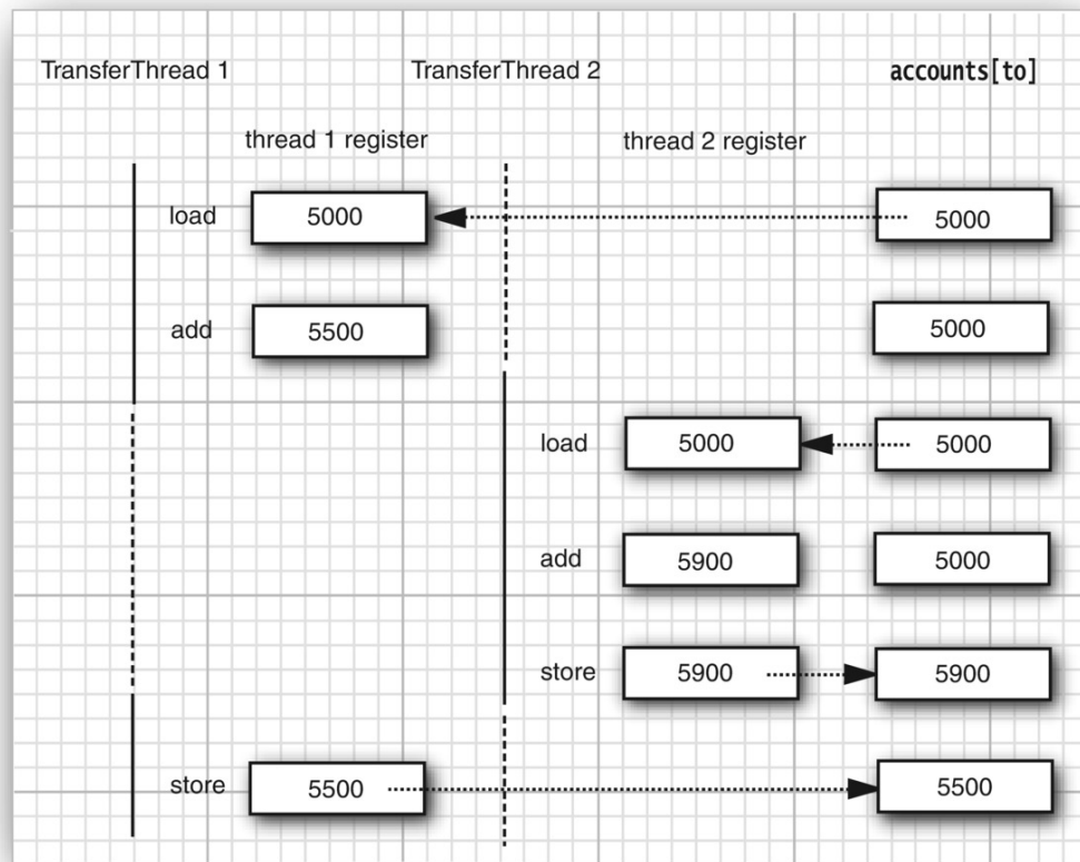
Figure 10.2: Simultaneous access by two threads
