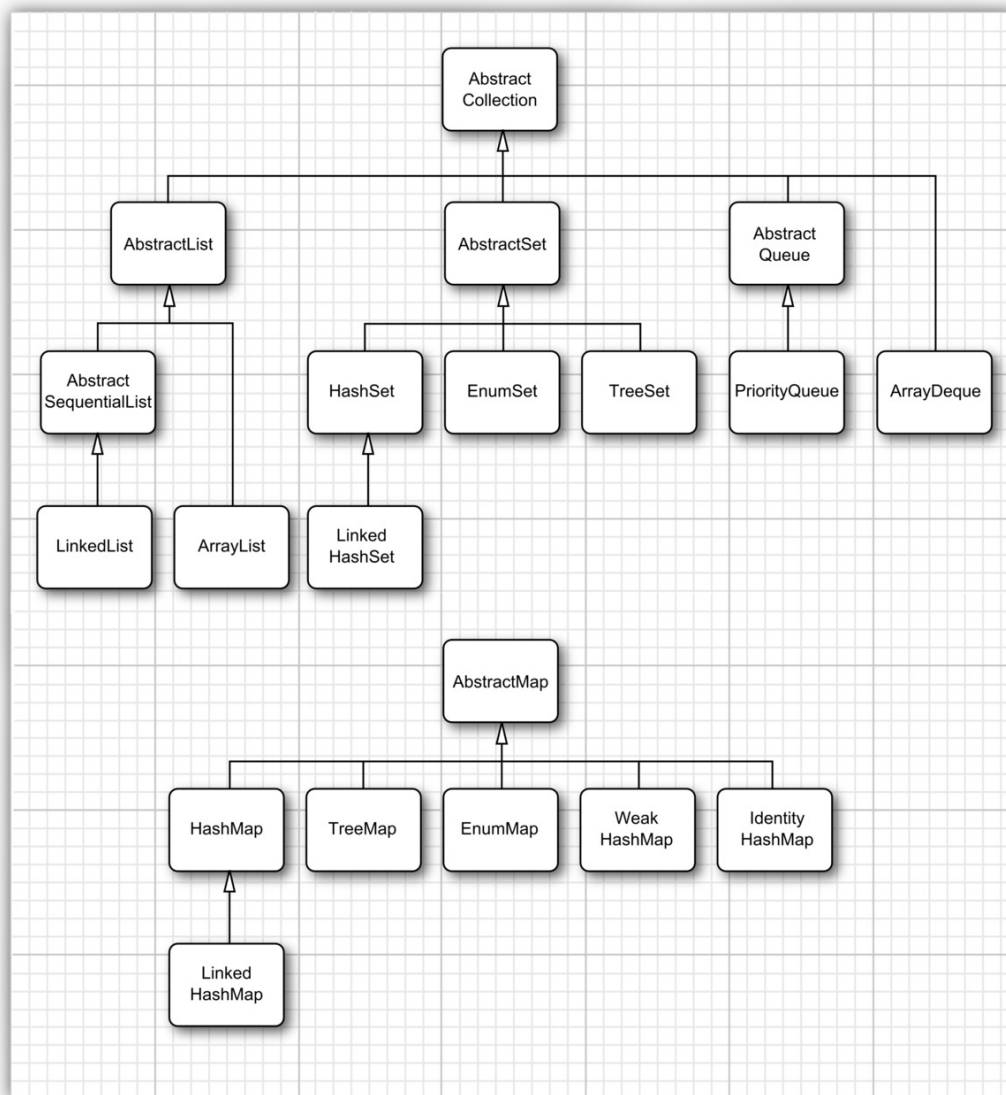
Figure 9.5: Classes in the Java Collections Framework
