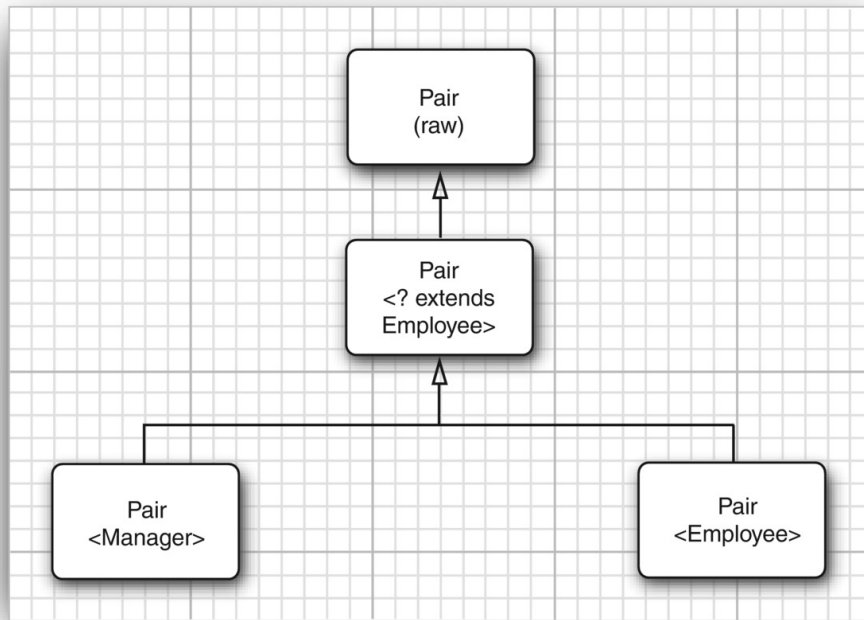
Figure 8.3: Subtype relationships with wildcards
