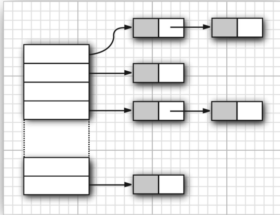
Figure 9.10: A hash table
