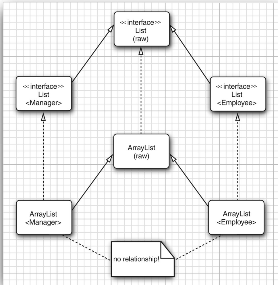
Figure 8.2: Subtype relationships among generic list types
