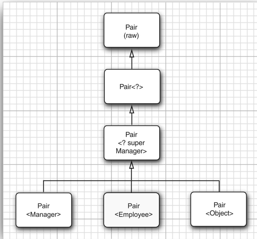
Figure 8.4: A wildcard with a supertype bound
