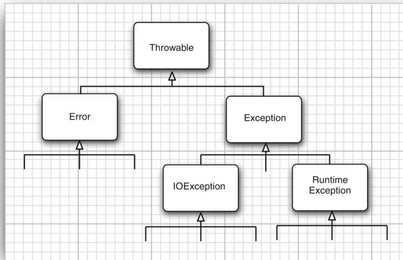
Figure 7.1: Exception hierarchy in Java
