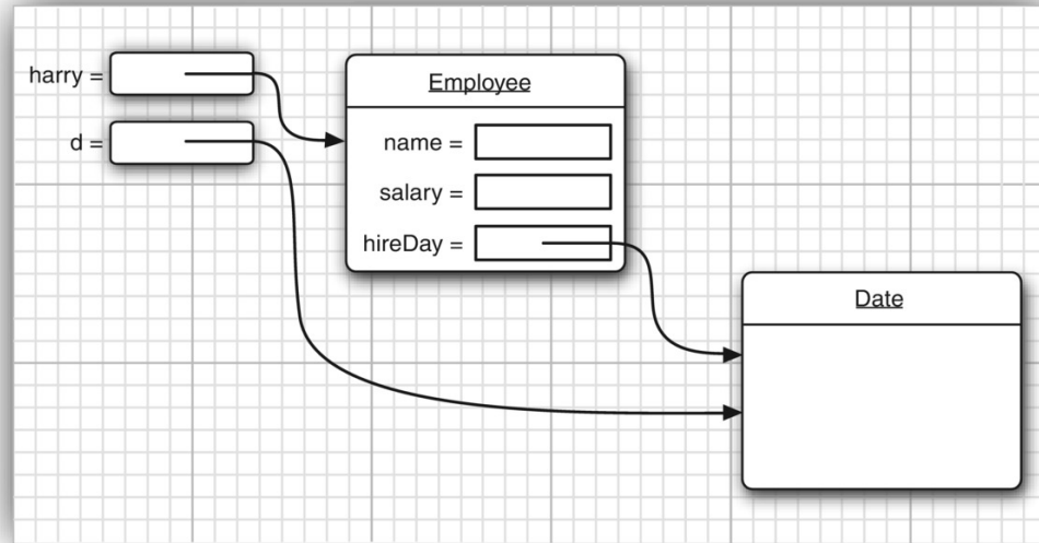
Figure 4.5: Returning a reference to a mutable instance field
