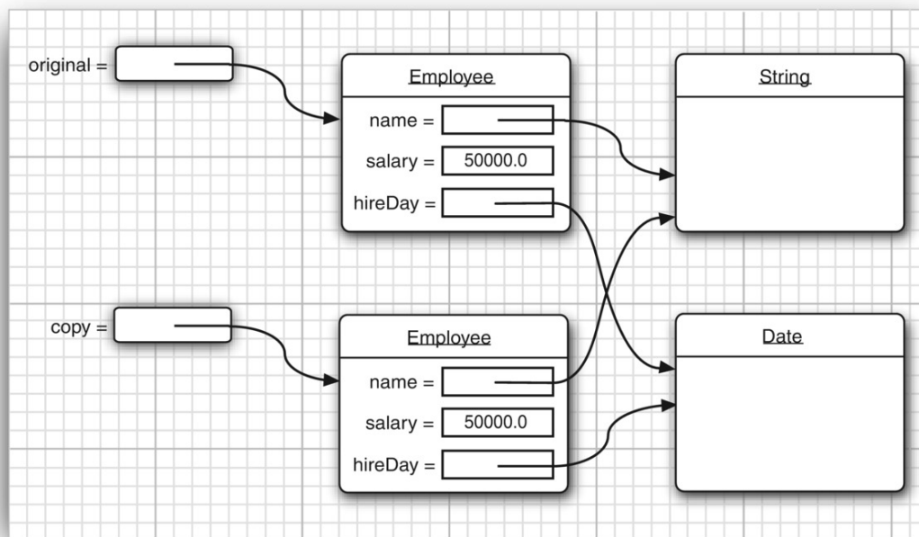
Figure 6.2: A shallow copy
