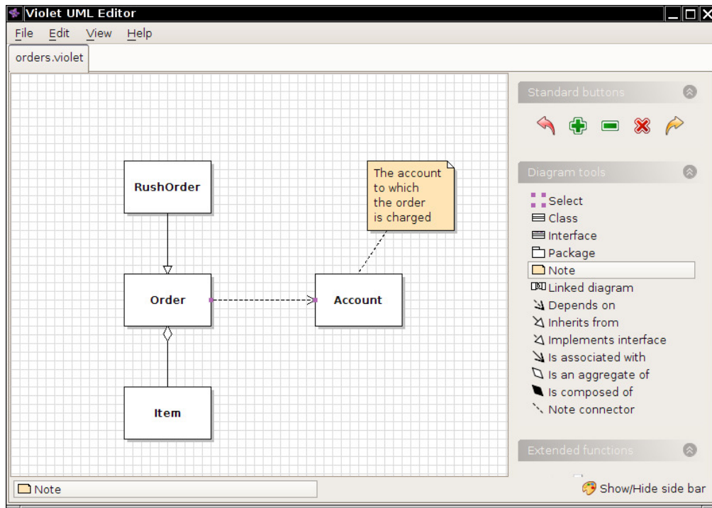
Figure 4.2: A class diagram
