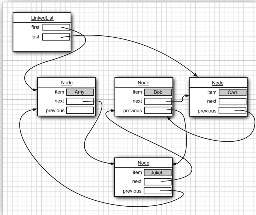
Figure 9.9: Adding an element to a linked list
