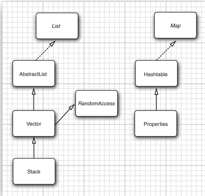
Figure 9.12: Legacy classes in the Java Collections Framework
