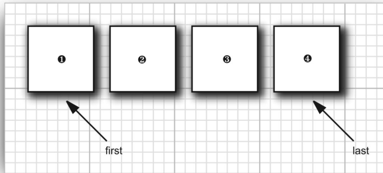
Figure 9.1: A queue
