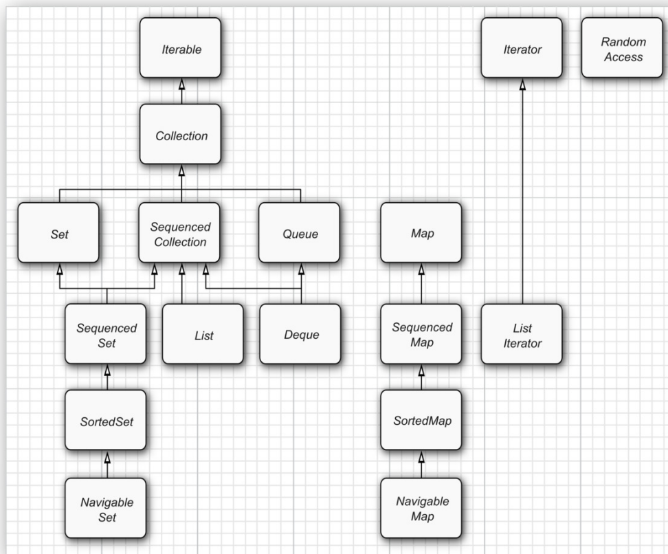
Figure 9.4: The interfaces of the Java Collections Framework
