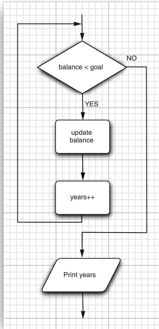
Figure 3.10: Flowchart for the while statement
