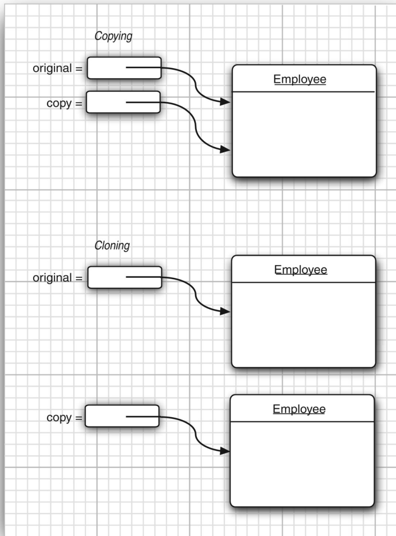
Figure 6.1: Copying and cloning
