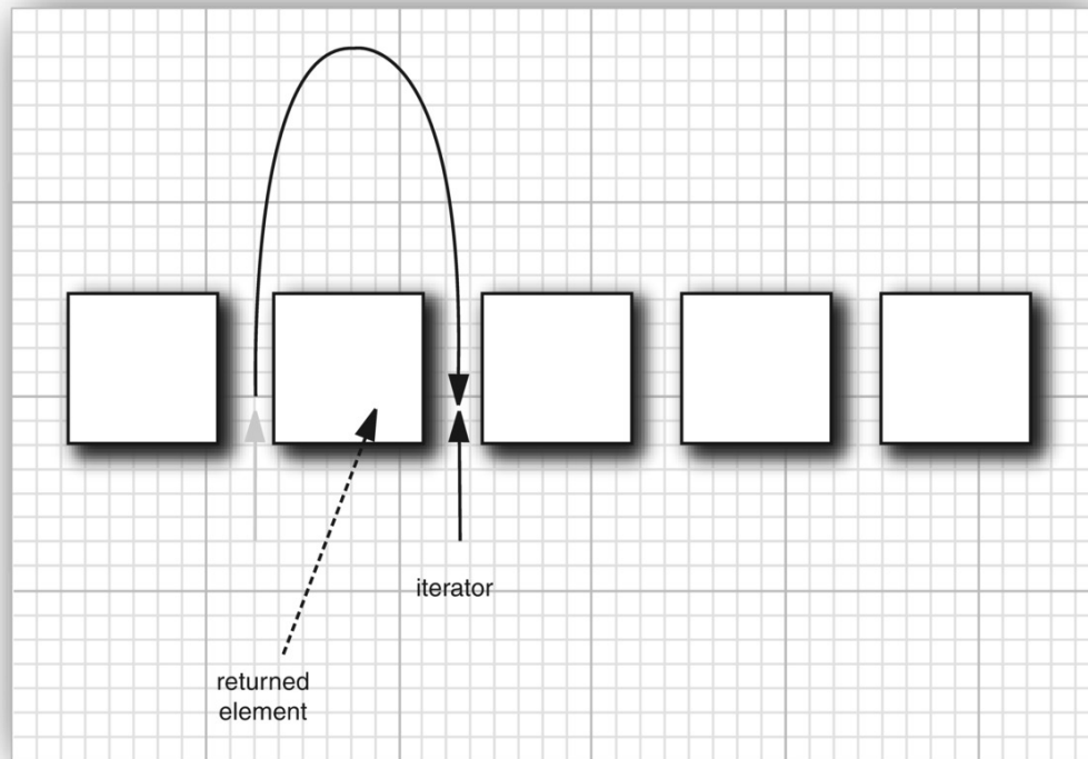
Figure 9.3: Advancing an iterator
