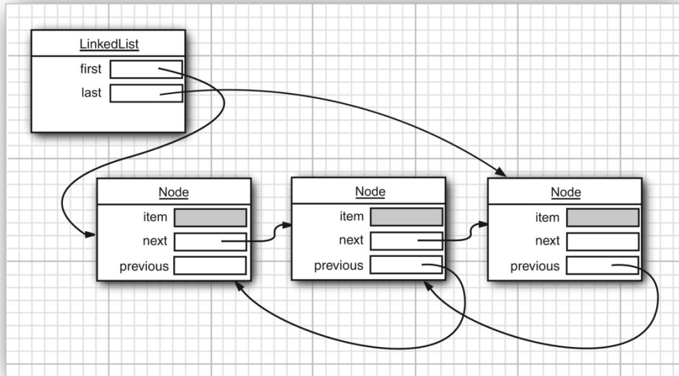
Figure 9.7: A doubly linked list
