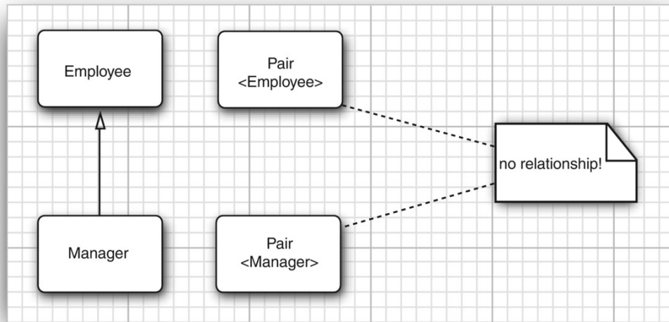
Figure 8.1: No inheritance relationship between Pair classes
