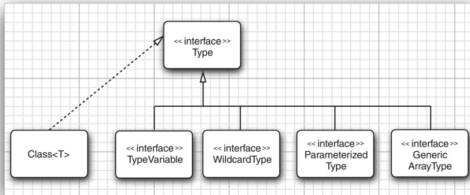
Figure 8.5: The Type interface and its descendants
