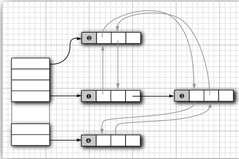
Figure 9.11: A linked hash table
