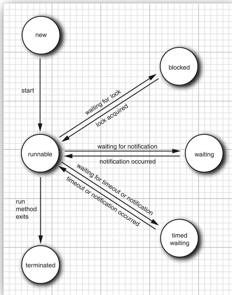
Figure 10.1: Thread states
