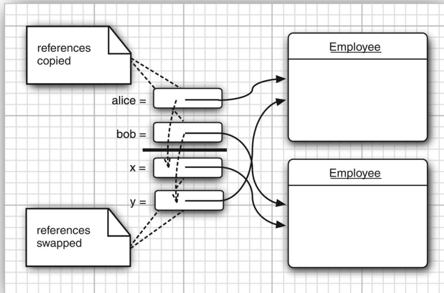
Figure 4.8: Swapping parameter variables has no lasting effect.
