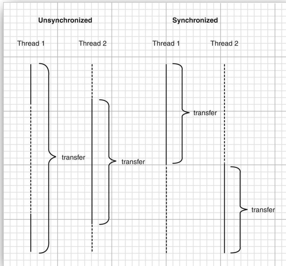
Figure 10.3: Comparison of unsynchronized and synchronized threads
